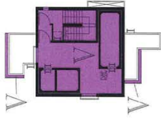
PLAN OF PUMP ROOM
