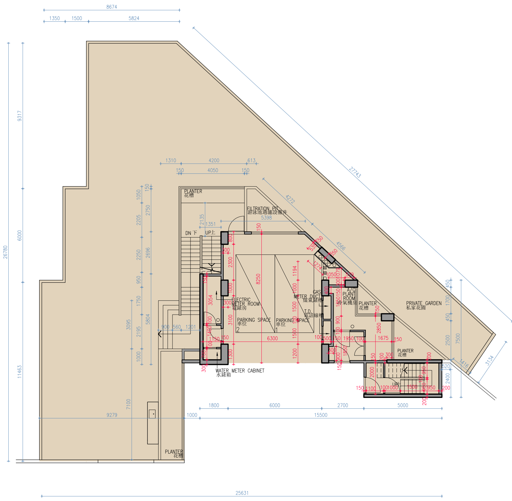
7 號洋房停車場平面圖 HOUSE 7 CAR PARK FLOOR PLAN
