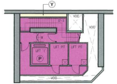
LIFT PIT PART PLAN
